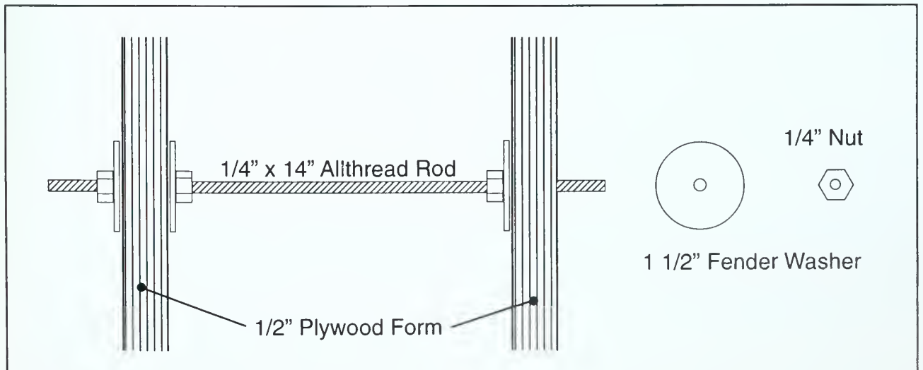
Figure 2. Allthread assembly.
